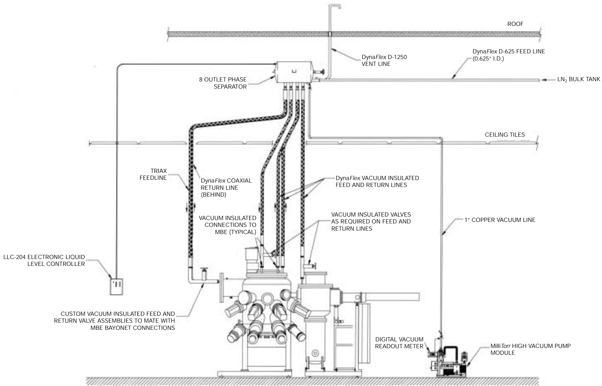
TYPICAL CLOSED LOOP LIQUID NITROGEN DynaFlex™ PIPING SYSTEM FOR MBE
